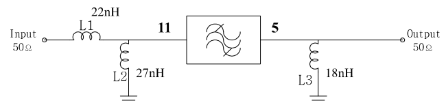
Matching Schematic
